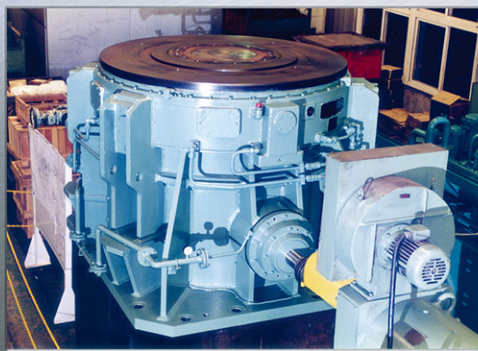
微粉炭破砕機用遊星歯車減速機の 無負荷試運転 No-Load Test Running for Pulverizer Gear Reducer
